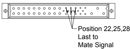
CONNECTOR DIMENSIONS
