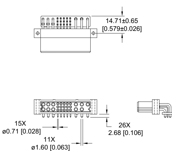
CONNECTOR DIMENSIONS
