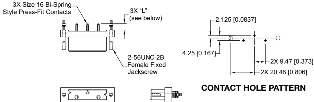
CONNECTOR DIMENSIONS
