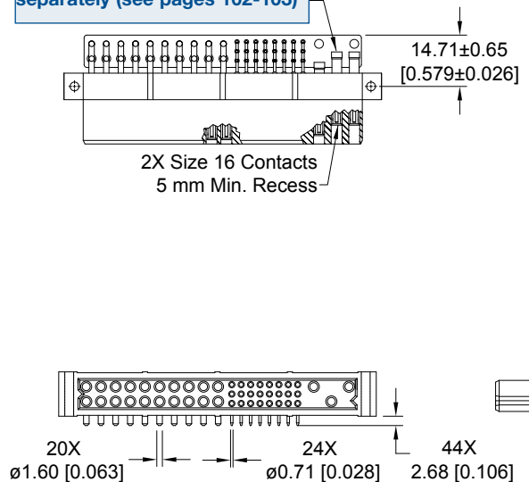
CONNECTOR DIMENSIONS
